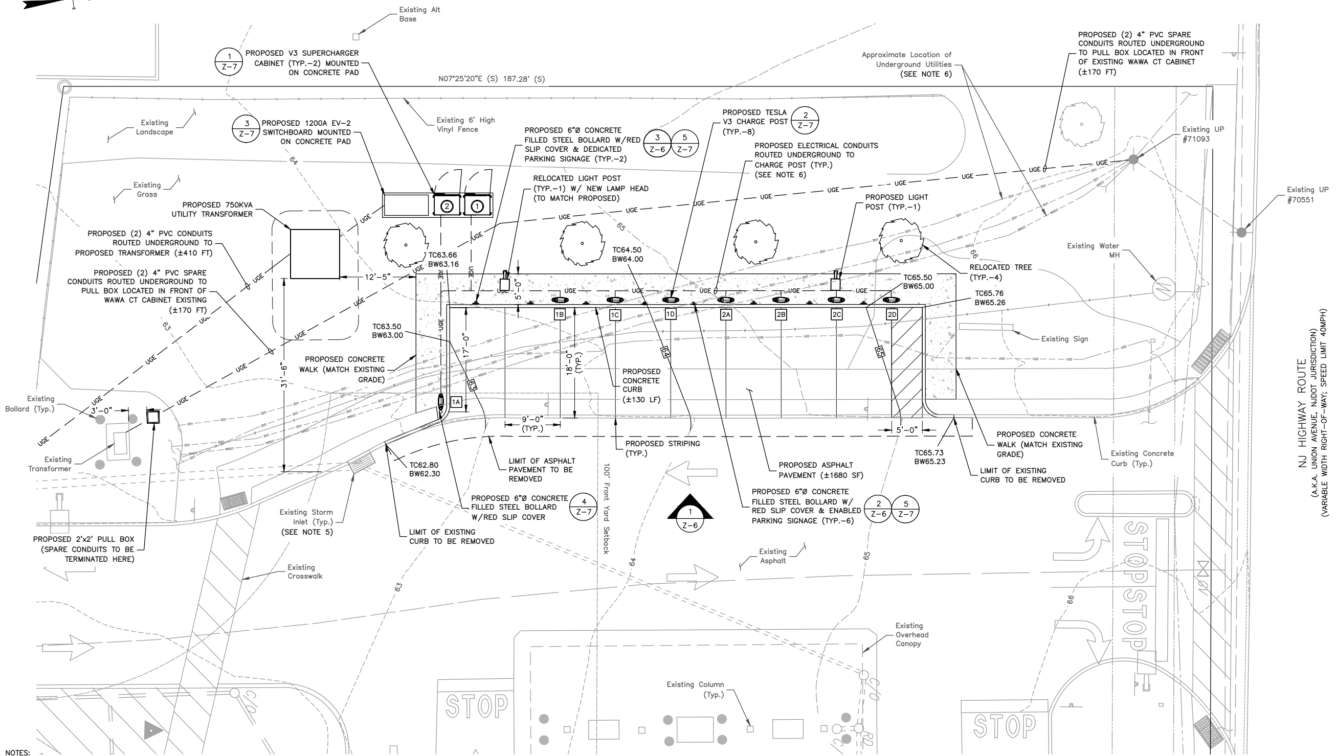
EQUIPMENT & PARKING PLAN 1 SCALE: 1/16"=1' FOR 11"x17" 1/8"=1' FOR 22"x34" 0' 4' 8' 16'
