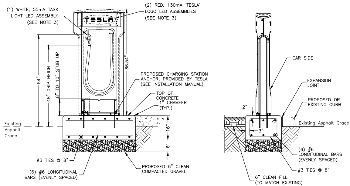
ILLUMINATED CHARGING STATION FOOTING DETAIL SCALE: N.T.S.
