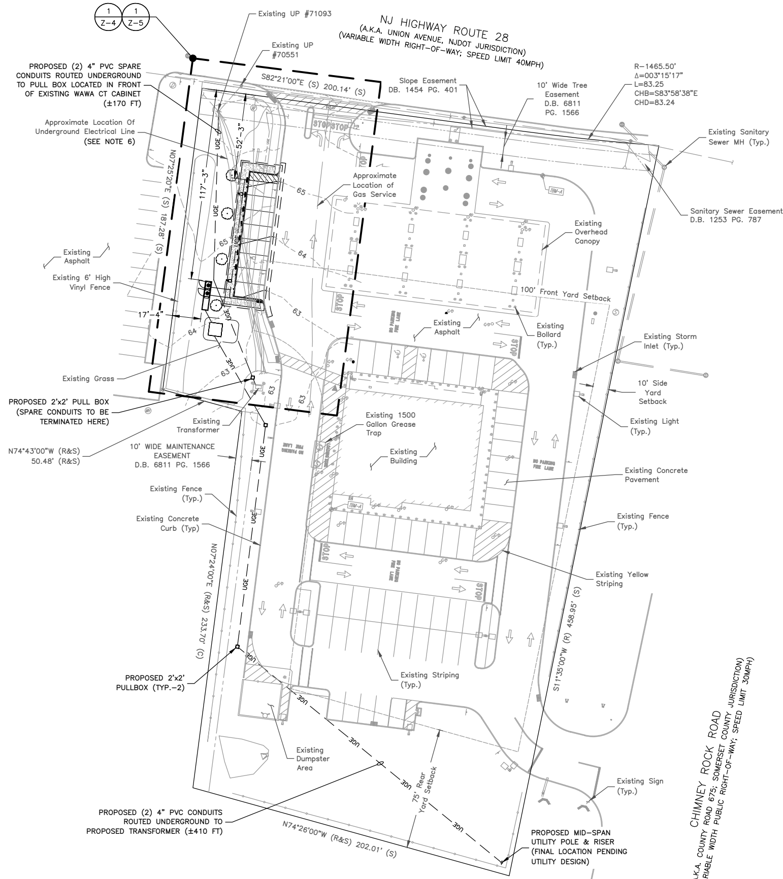
SITE PLAN SCALE: 1"=60' FOR 11"x17" 1"=30' FOR 22"x34" 0' 30' 60'
